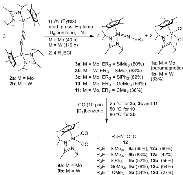
Scheme 5. Photolysis of 2 in the presence of excess equivalents of \text{R}_3\text{ECl} and subsequent nitrene-group transfer from 3 , 10 , and 11 to CO. Yields of products are relative to 2 and based on durene as an internal standard. [8]
